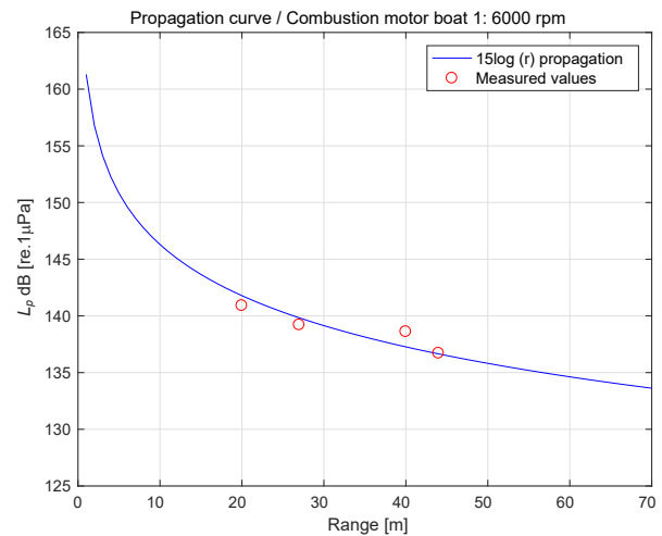
Fig. 8. Comparison between calculated transmission loss, distance and those levels obtained during the measurement for combustion boat 1, at velocity 6000 rpm.
