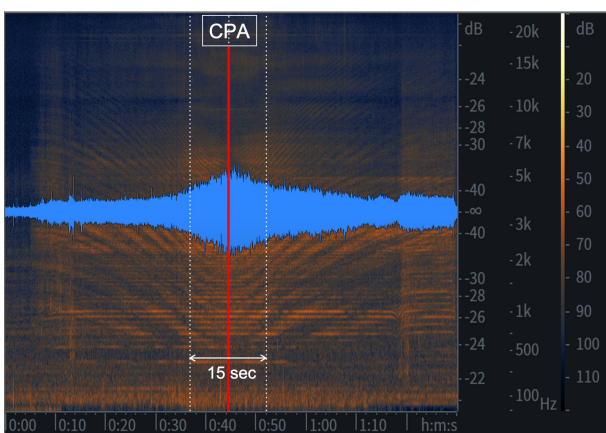
Fig. 6. Waveform and spectrogram. Example of a 15-second time interval centered on the point of the shortest distance from the boat to the hydrophone or CPA.
