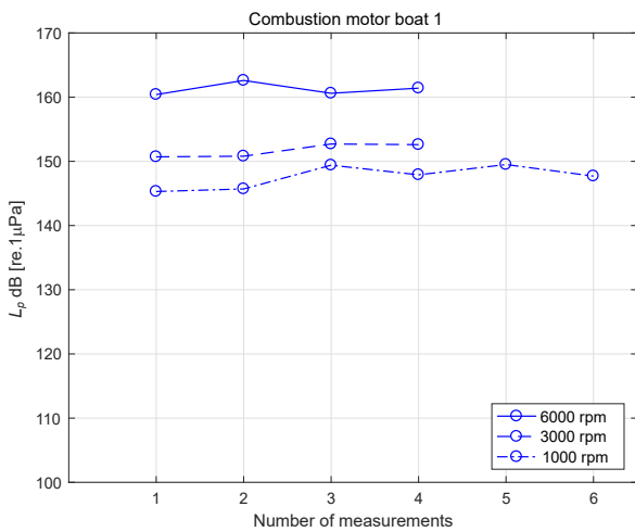
Fig. 12. Source levels L_{p,1m} , obtained for the combustion motor boat 1.
