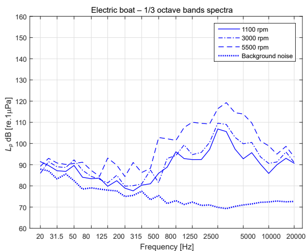
Fig. 17. 1/3 octave bands spectra of the electric motor boat, for the three velocities evaluated. Likewise, the background noise registered in the area is shown.
