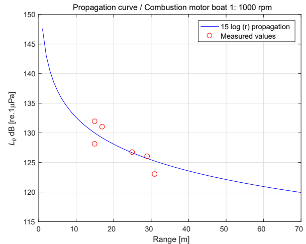
Fig. 7. Comparison between calculated transmission loss, distance and those levels obtained during measurement for the combustion boat 1, at velocity 1000 rpm.
