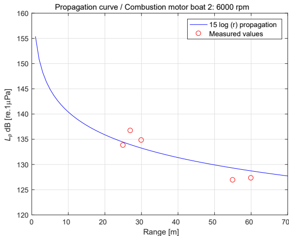
Fig. 10. Comparison between calculated transmission loss, distance and those levels obtained during the measurement for combustion boat 2, at velocity 6000 rpm.
