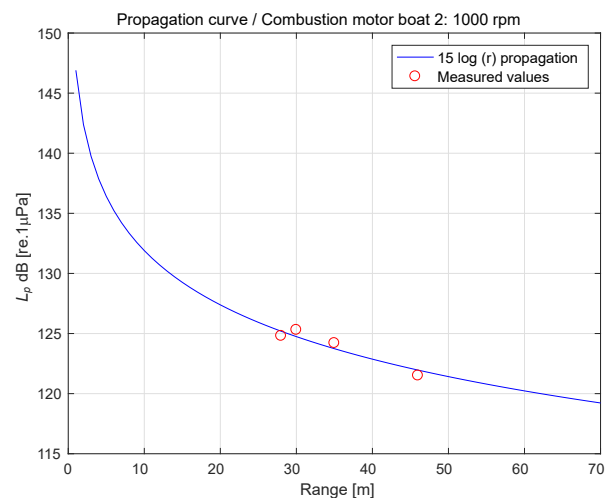
Fig. 9. Comparison between calculated transmission loss, distance and those levels obtained during the measurement for combustion boat 2, at velocity 1000 rpm.
