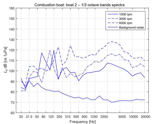
Fig. 19. 1/3 octave bands spectra of the combustion motor boat 2, for the three velocities evaluated. Background noise measured in the place is also shown.
