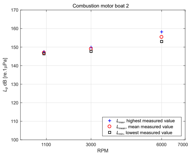
Fig. 16. Average source levels L_{p,1m} of the combustion motor boat 2, together with the highest and lowest levels, for the three evaluated velocities.
