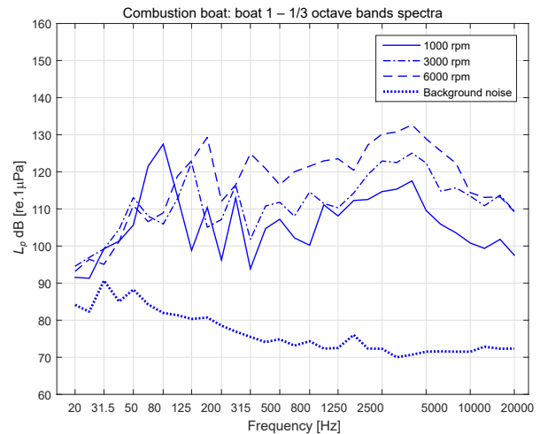
Fig. 18. 1/3 octave bands spectra combustion motor boat 1, for the three velocities evaluated. Background noise measured in the area is also shown.
