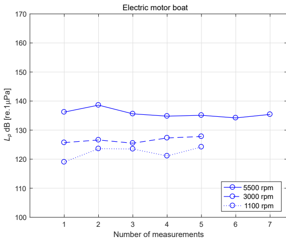
Fig. 11. Source levels L_{p,1m} , obtained for the electric motor boat.
