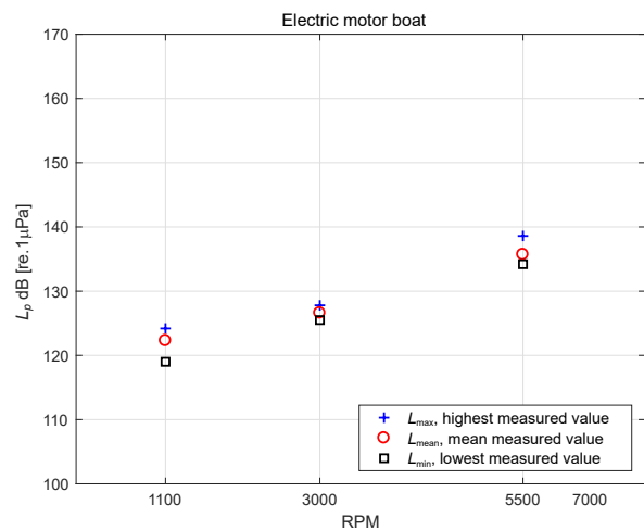
Fig. 14. Average source levels L_{p,1m} of the electric motor boat, together with highest and lowest levels for the three evaluated velocities.
