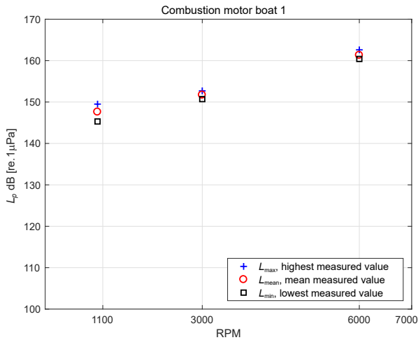
Fig. 15. Average source levels L_{p,1m} of the combustion motor boat 1, together with the highest and lowest levels, for the three evaluated velocities.
