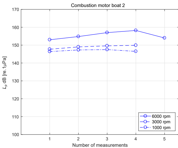
Fig. 13. Source levels L_{p,1m} , obtained for the combustion motor boat 2.
