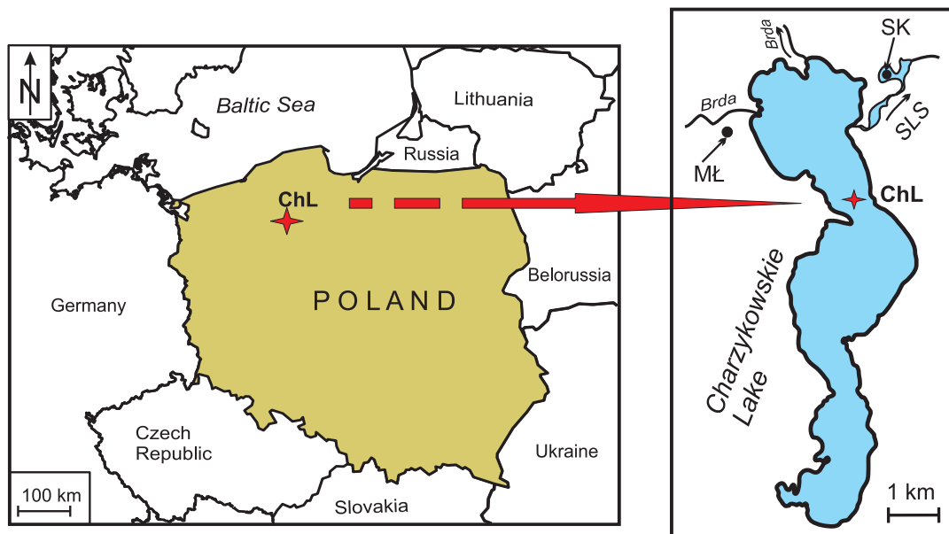
Text-fig. 1. Location of Charzykowskie Lake. ChL – drilling point of sediment core; SLS – Seven Lakes' Stream; MŁ – Małe Łowne peat bog; SK – Skrzyńska Lake (Apolinarska et al. 2012).
