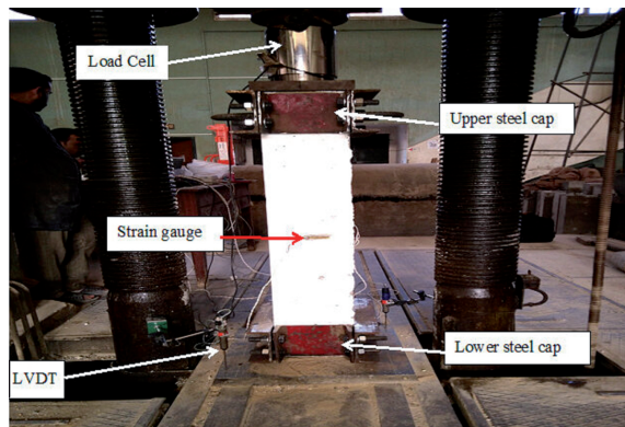
Fig. 2. Details of test setup
