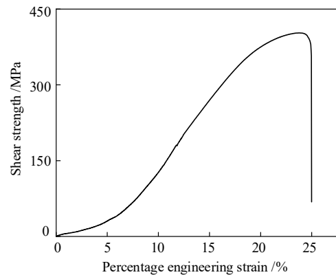
Fig. 16. Tensile shear stress-strain curve
