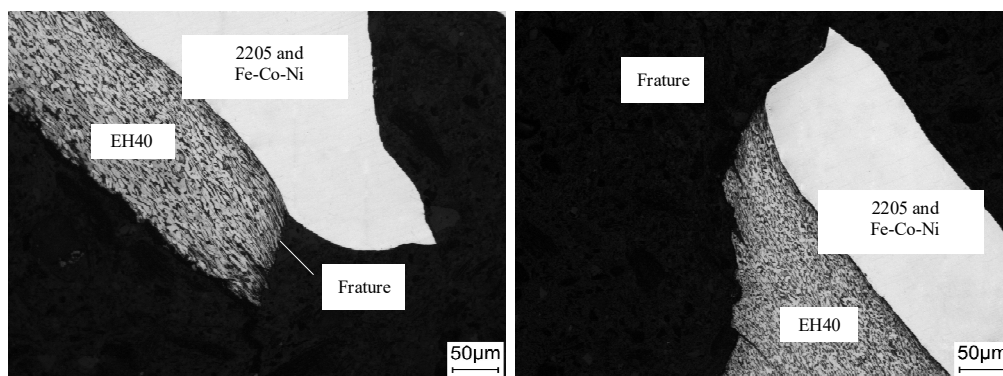
Fig. 18. Fracture microstructure
