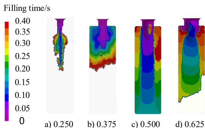
Fig. 7. Coating process at different suction layer width ratios
