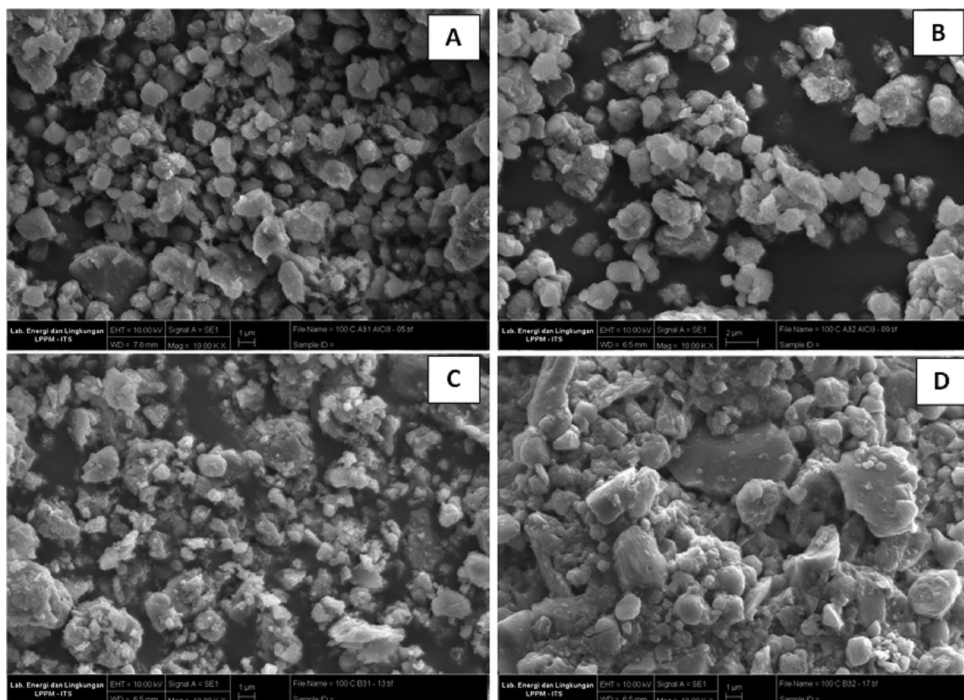
Fig. 5. Scanning Electron Microscopy (SEM) Characterization Results of Zeolite with magnification of 10.00 KX A) A31 \text{AlCl}_3 , B) A32 \text{AlCl}_3 , C) B31, and D) B32
