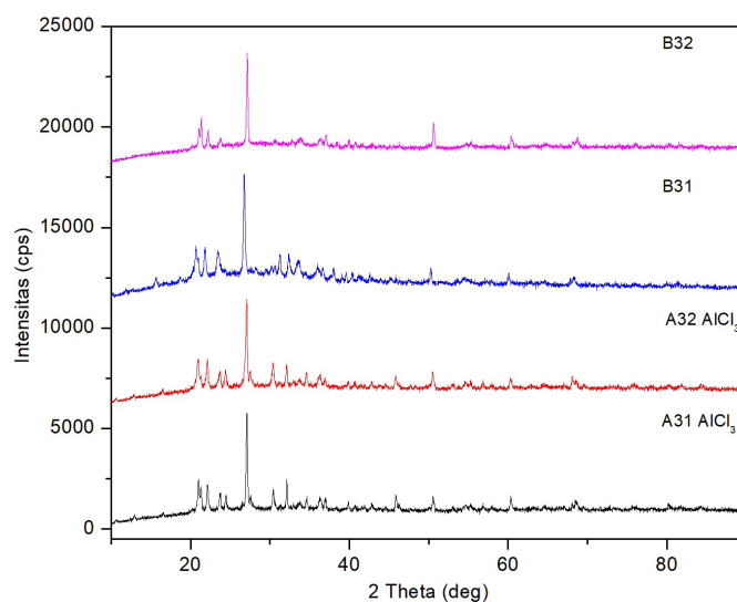
Fig. 2. The results of the X-Ray Diffraction (XRD) characterization of zeolite samples
