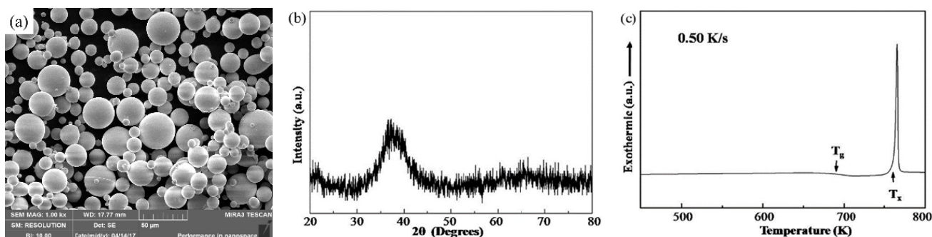
Fig. 3. (a) Scanning electron micrograph; (b) XRD pattern; (c) DSC curve of the raw Zr55Cu30Al10Ni5 amorphous powders
