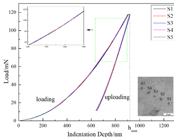
Fig. 7. P-h curves of bulk Zr55Cu30Al10Ni5 amorphous alloy samples sintered at 705K
