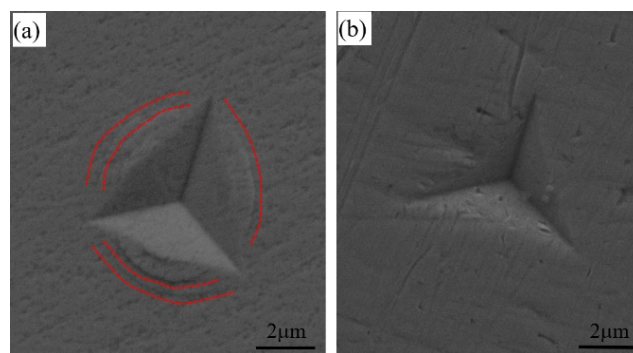
Fig. 8. Indentation morphology of the bulk Zr55Cu30Al10Ni5 amorphous alloy sintered at different temperatures: (a) 675K, (b) 705K
