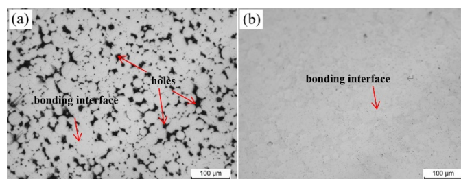
Fig. 5. Microstructures of the bulk Zr55Cu30Al10Ni5 amorphous alloy sintered at different temperatures: (a) 675K, (b) 705K
