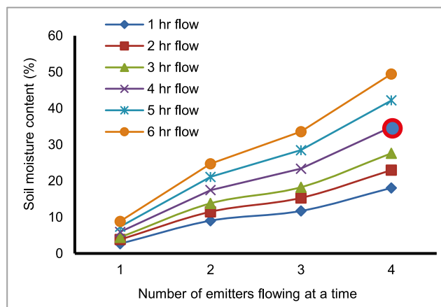
Fig. 3. Soil moisture content observed at 120 cm vertical depth and 100 cm horizontal distance from emission points; source: own study
