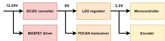
Fig. 3. Power supply diagram
