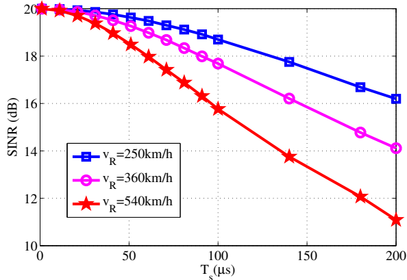
Fig. 3. SINR versus symbol duration for different train speeds with SNR = 20 dB
