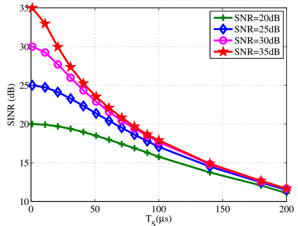
Fig. 4. SINR versus symbol duration for v_R = 540 \text{ km/h} with different SNRs.
