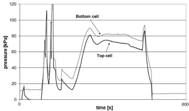
Fig. 10. Conditioned pozzolanic soil. Pressure recorded by the sensors installed in the tank
