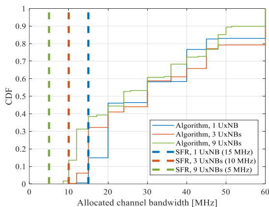
Fig. 8. Simulation results of allocated channel bandwidth obtained for the algorithm and SFR scheme in terrestrial and aerial 3GPP RMA deployment
