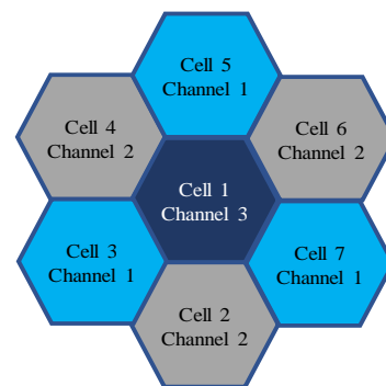
Fig.5. The frequency planning and power allocation for the SFR scheme [14]
