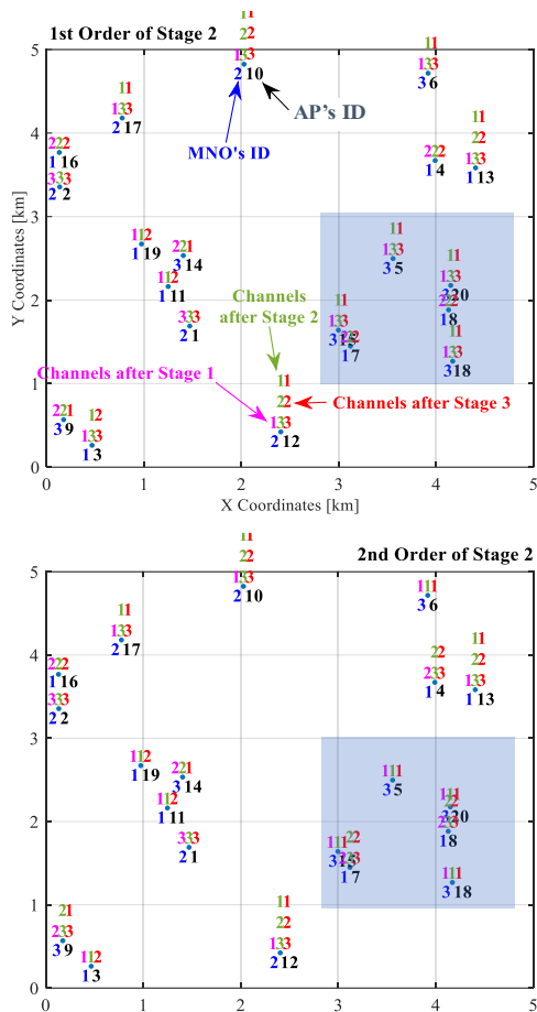
Fig. 4. Results of simulation verification of the consecutive stages of the algorithm
