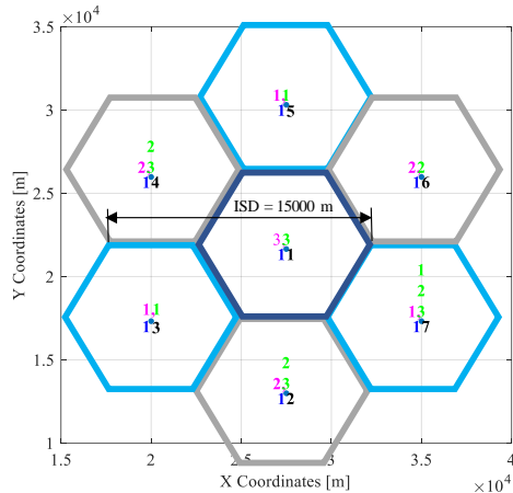
Fig. 6. Geometry of the assumed simulation scenario and example outcome of the algorithm's calculations
