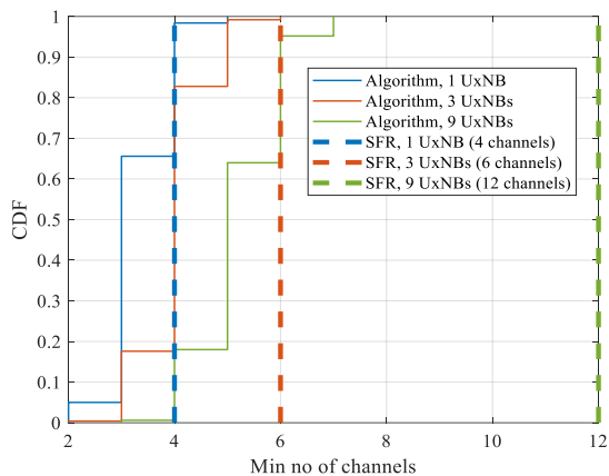
Fig. 7. Simulation results of minimal number of channels obtained for the algorithm and SFR scheme in terrestrial and aerial 3GPP RMA deployment
