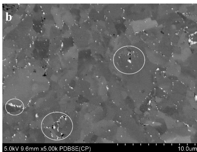
Fig. 9. a) Structural image after extruding composite with 2% iron content, b) Structural image after extruding composite with 5% iron content
