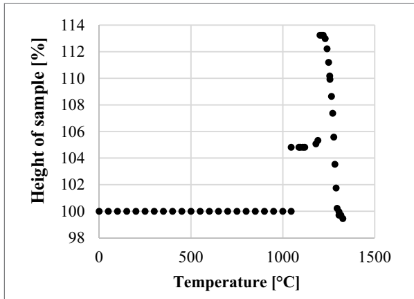
Fig. 10. Change in the height of the tested Al-Fe composite capsule (2% iron powder) due to temperature
