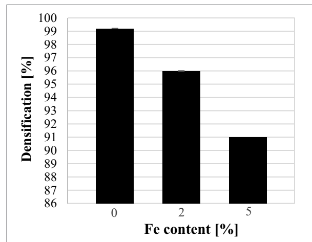
Fig. 12. Bar graph of densification of Al-Fe composites as a function of Fe content
