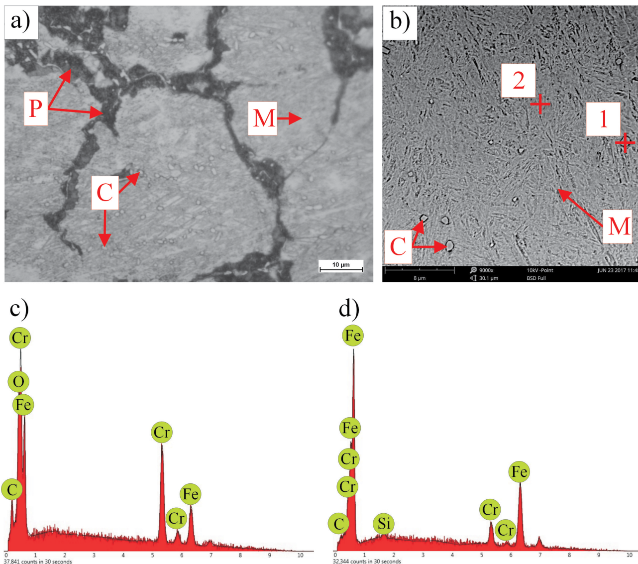
Fig. 7. Example microstructure of the working layer of the bimetallic casting X46Cr 13 steel – grey cast iron; Cr (Fe) carbides (C), martensite (M) and pearlite (P): a) OM, mag. 1000 \times , b) SEM, mag. 9000 \times ; 1 and 2 as points of EDS analysis, c) the result of EDS in point 1 from Fig. b and d) the result of EDS in point 2 from Fig. b
