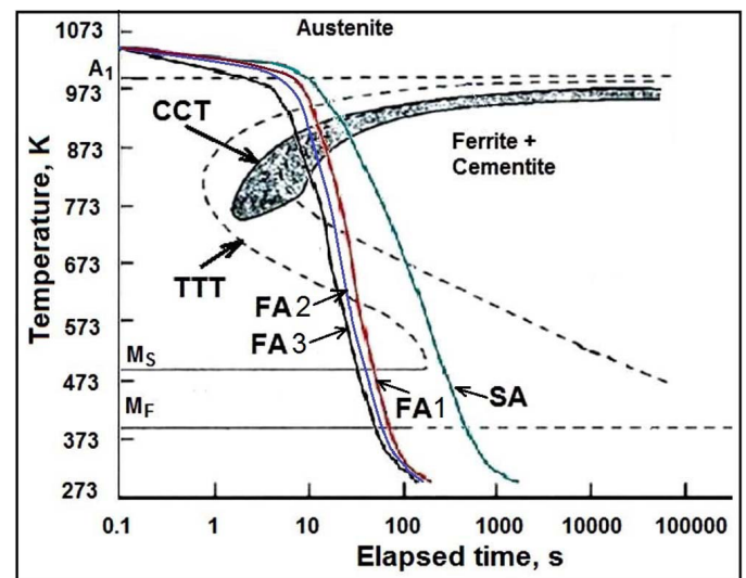
Fig. 1. Cooling curves superimposed on the CCT diagram of AISI 1080 Steel
