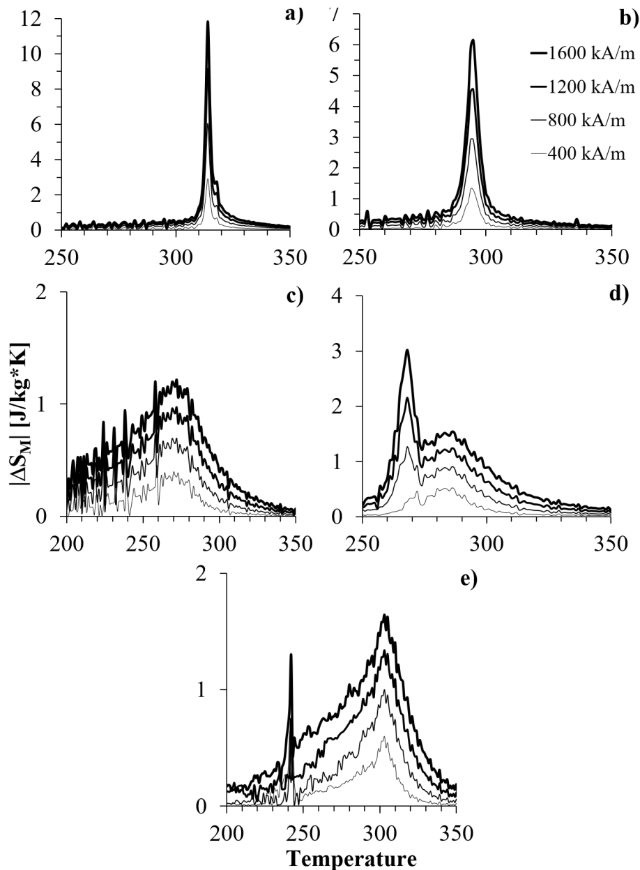
Fig. 2. Magnetic entropy changes calculated for \text{Ni}_{50}\text{Mn}_{18.75}\text{Cu}_{6.25-x}\text{Pb}_x\text{Ga}_{25} ; a) 1, b) 2, c) 3, d) 4, e) 5 at.% alloys
