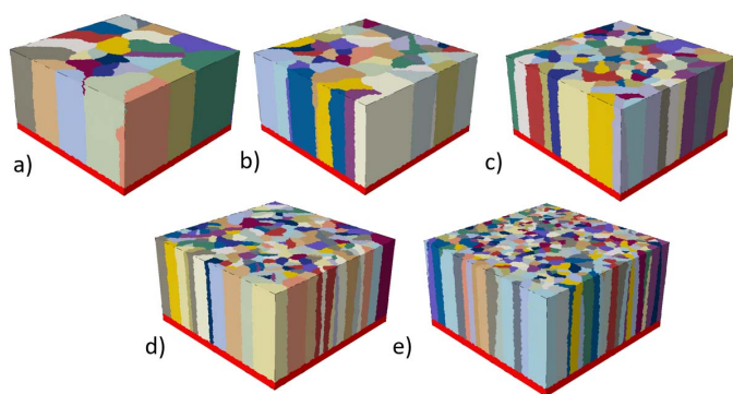
Fig. 6. Generated, with the pentagonal random CA neighbourhood, set of digital models of TiN thin-films with a) 25 b) 50 c) 100 d) 200 and e) 400 columns
