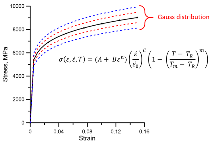
Fig. 11. Schematic representation of flow stress curves generated with the Gaussian distribution function (where: A, B, C, n, m – material constants, \sigma – plastic flow stress, \varepsilon – equivalent plastic strain, \dot{\varepsilon} – equivalent plastic strain rate, \dot{\varepsilon}_0 – reference equivalent plastic strain rate, T_m – melting temperature, T_R – transition temperature)
