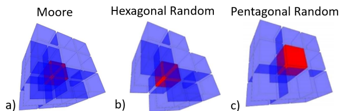
Fig. 2. a) Moore, b) hexagonal random and c) pentagonal random neighbourhoods of the CA cell marked in red
