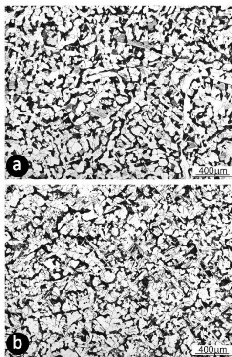
Fig. 4. Microstructure of G20Mn5 cast steel without heat treatment, a – non-modified, b – modified with REM
