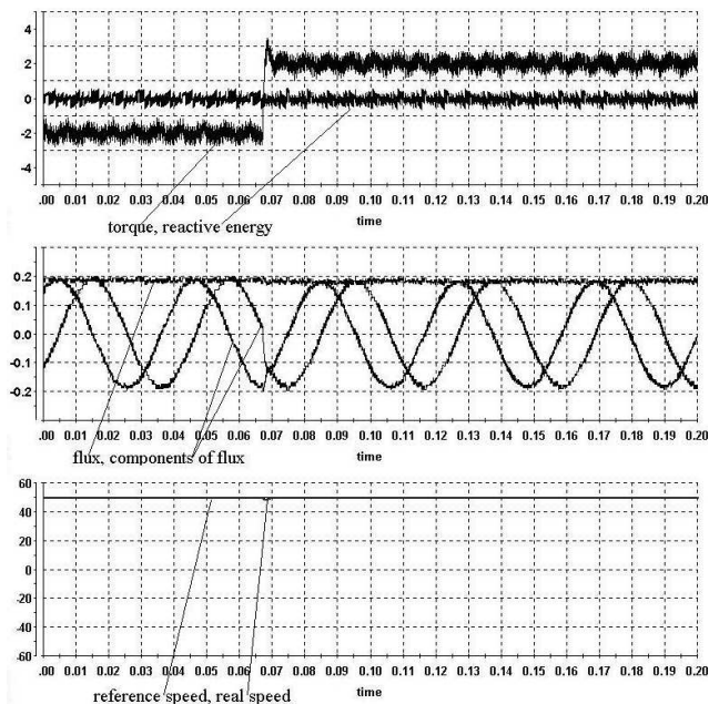
Fig. 8. Time waveforms of torque, reactive energy, flux and angular speed during torque reversal ( -2 Nm; 2 Nm) for BLDCM (time 10 ms/div)
