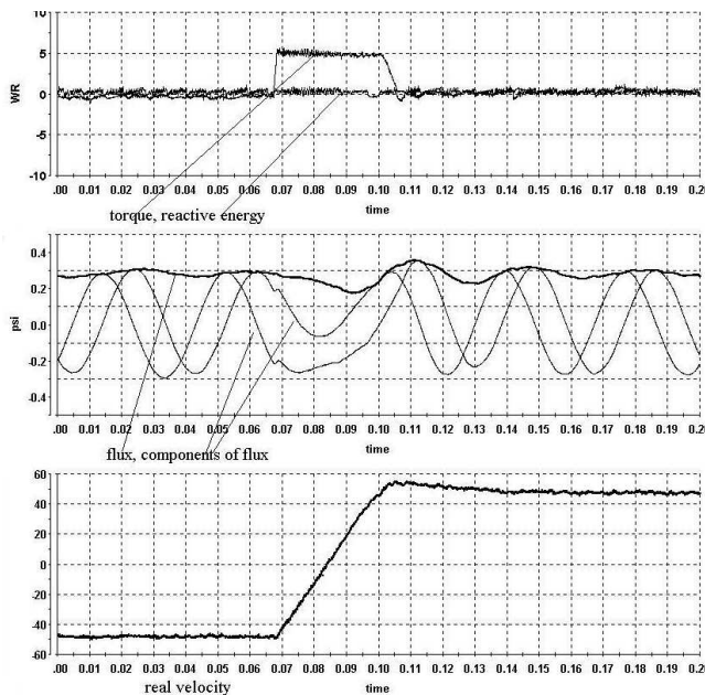
Fig. 9. Time waveforms of torque, reactive energy, flux and angular speed during speed reversal ( -50 rd/s; 50 rd/s) for PMSM (time 10 ms/div)
