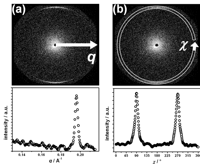
Fig. 6. A demonstration of X-ray diffraction principles using the liquid crystal, 8CB. (a) Radial averaging of the image over all azimuthal angles (top) results in a plot of intensity versus scattering vector q . (b) Azimuthal integration of a raw image (top) about a fixed radial position results in a plot of intensity versus orientation angle \chi
