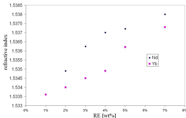
Fig. 13. Effect of RE ( \text{Nd}_2\text{O}_3 and \text{Yb}_2\text{O}_3 ) doping on the value of refractive index
