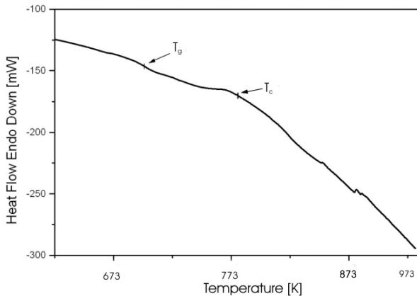
Fig. 2. DSC curve of 28Al-25Si glass
