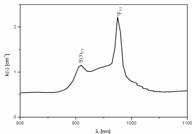
Fig. 6. Spectral absorption coefficient k(\lambda) of \text{Yb}^{3+} (2 wt%) glass
