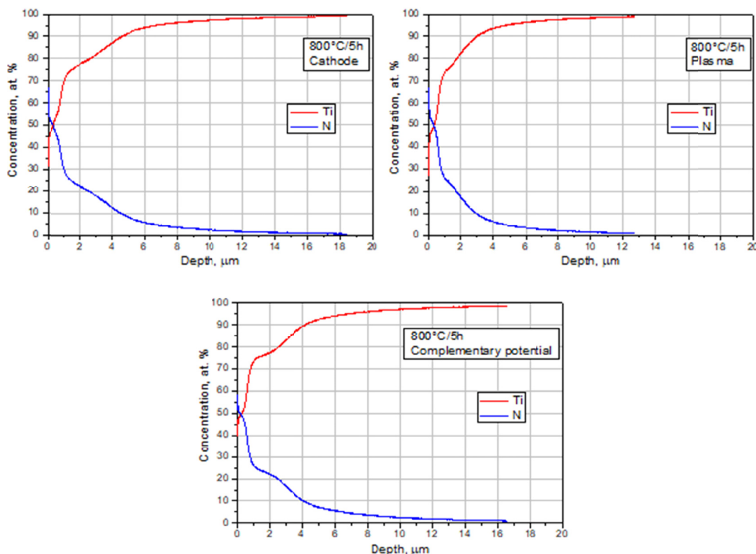
Fig. 3. Nitrogen and titanium concentration distribution profiles (Glow Discharge Optical Emission Spektroskopy) for nitrided samples
