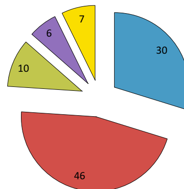
Text-fig. 11. Trophic nuclei of the Lower Maastrichtian B. obtusa and B. sumensis zones at Krons Moor
