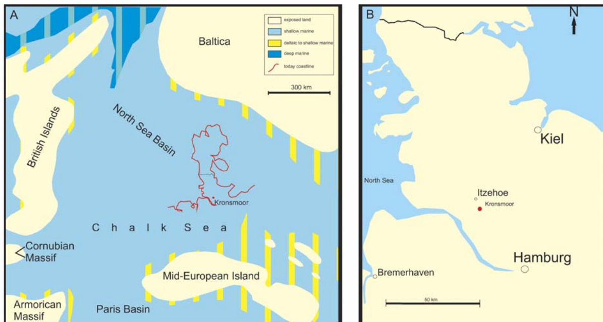
Text-fig. 1. A – Palaeogeographic map of the Late Cretaceous Chalk Sea during the Cenomanian to Maastrichtian, modified after (Vejbæk et al. 2010); B – Map of northern Germany showing the position of the Kronsmoor section (red dot)
