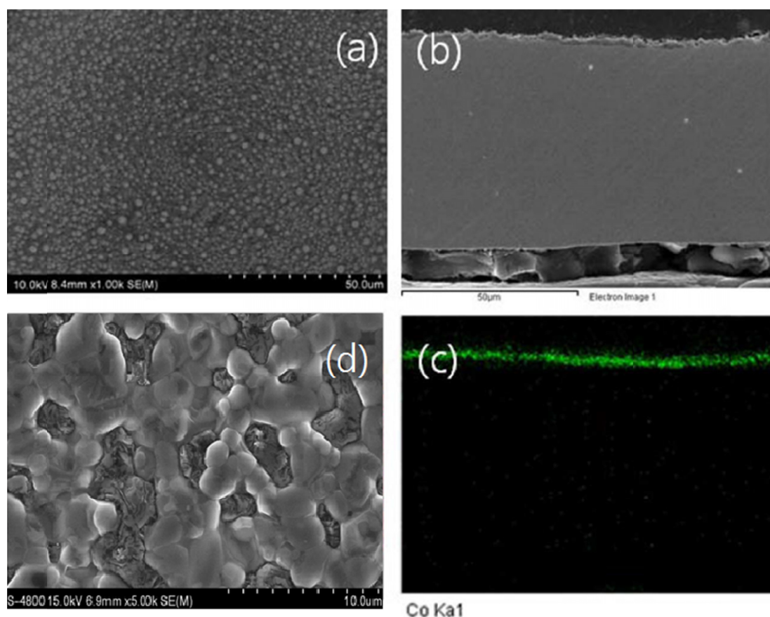
Fig. 3. SEM images for (a) surface of Co layer on Rh foil, (b) cross section images for Co coated Rh foil. Mapping of EDS for (c) Co layer in SEM image of (b), and (d) surface of Co-layer after annealing at 1100^{\circ}\text{C} for 3 h
