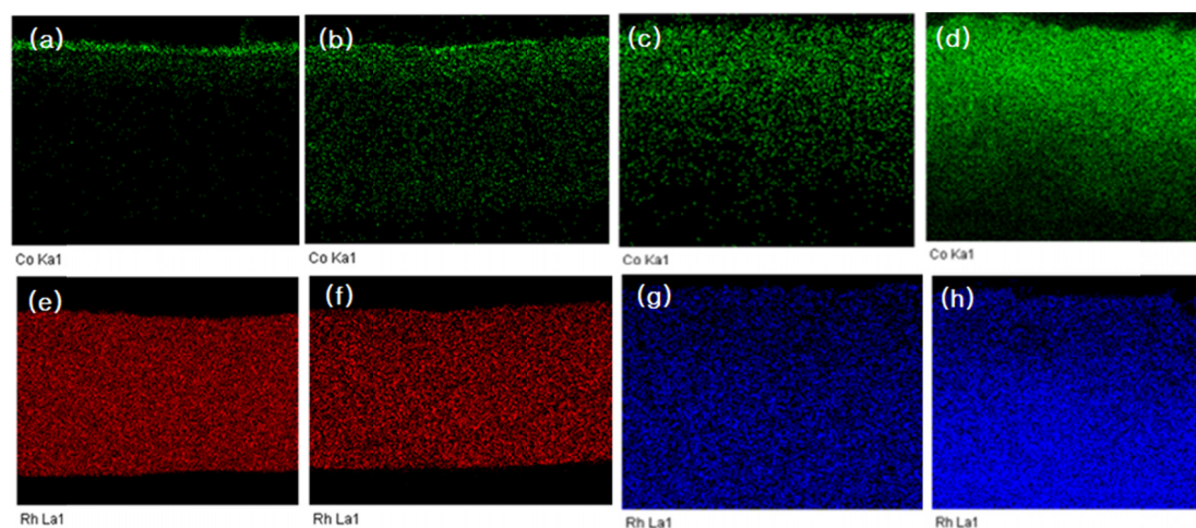
Fig. 4. Mapping of EDS for Co layer annealed under low vacuum using Ar inert gas at 1100^{\circ}\text{C} for (a) 1 h, (b) 5 h, and at 1200^{\circ}\text{C} for (a) 3 h, and (b) 5h. (e),(f),(g), and (h) are those of Rh layer
