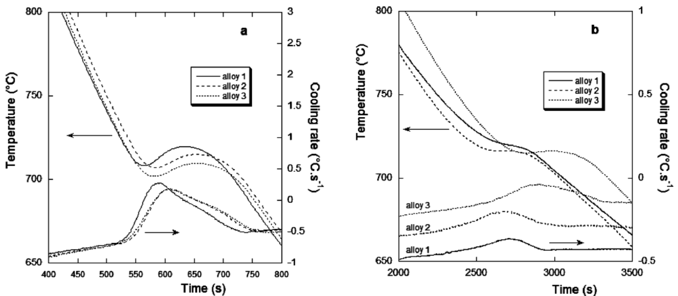
Fig. 6. Cooling curves and their derivative showing the peak associated to the eutectoid reaction when alloys 1, 2 and 3 are cast in TA cups (a) and keel-blocks (b). Note that the cooling rate curves have been shifted of arbitrary amounts in b for clarity (only the shape of the peak is of interest here)
