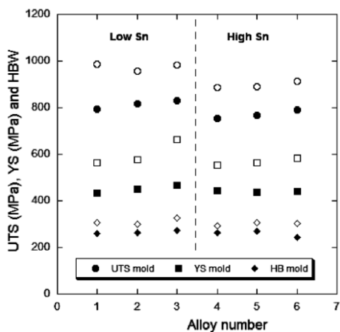
Fig. 8. Values of UTS, YS and HBW for the six alloys investigated. Solid and open symbols refer to mould and air cooled keel-blocks respectively
