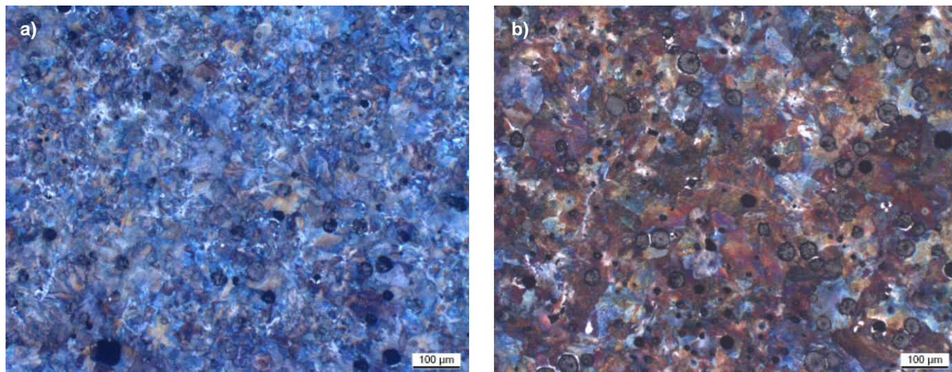
Fig. 7. Micrographs of alloys 6 cast in TA cup (a) and keel-block (b)
