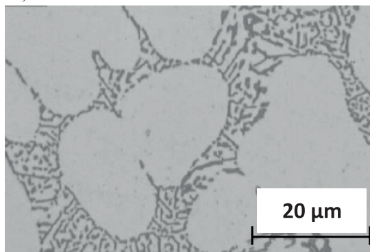
Fig. 5.-a) Microstructure of as-cast Al-6%Si alloy refined by Ti-6Al-4V by mesh 50 with 0.15wt%. Average grain size is about 6\mu\text{m} and silicon length was reduced to a few micrometers and distributed homogeneously in the section of the specimen. b) Tensile curve at strain rate of 10\text{-}1\text{ s}^{-1} in room temperature. The maximum strength is about 492\text{MPa} and fracture occurred at the elastic limit with 7.25\% elongation. c) The same microstructure with more magnification. The morphology of the eutectic silicon is changed from needle-plate to a fibrous form.
