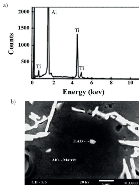
Fig. 2. a) SEM/EDX micro-analyzing shows that TiAl_3 compound in the microstructure. b) Microstructure of as-cast Al-6% Si alloy refined by Ti-6Al-4V inoculant alloy by scanning electron microscope (SEM)
