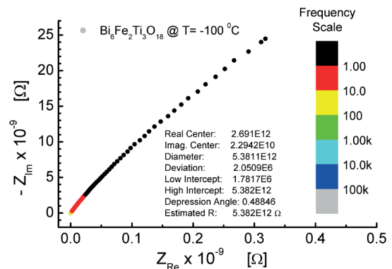
Fig. 5. Impedance diagrams in the complex Z''-Z' plane measured for \text{Bi}_6\text{Fe}_2\text{Ti}_3\text{O}_{18} ceramics at temperature T=0^\circ\text{C} (a), T=-100^\circ\text{C} (b); isotropic (a) and free scale (b) was used for data presentation
