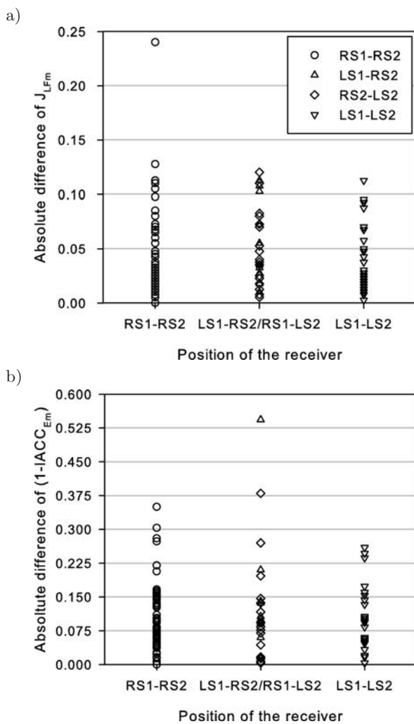
Fig. 7. Absolute differences between the values of: a) J_{LFm} , and b) ( 1-IACC_{Em} ), for the two source positions at the reception points for all concert halls. The various symbols of the reception points take into account how these see the two sources: both on the right (RS1-RS2), one on the right-hand side and another on the left or vice versa (RS1-LS2, LS1-RS2), or both on the left (LS1-LS2).
