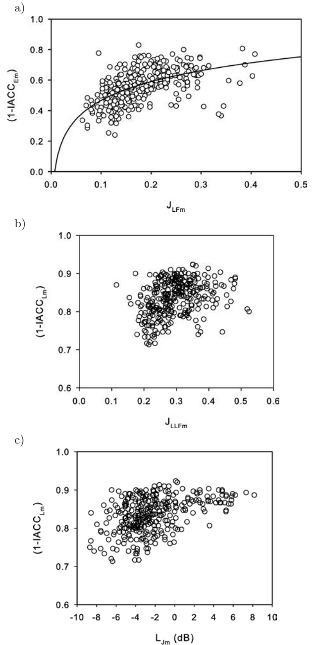
Fig. 9. a) (1-IACC_{Em}) versus J_{LFm} and the line of the logarithmic fit; b) (1-IACC_{Lm}) versus J_{LLFm} ; c) (1-IACC_{Lm}) versus L_{Jm} , where all values are given for all individual positions in the halls with the two source positions and two configurations of the stages.
