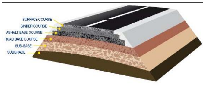
Fig. 1. Typical pavement layers
