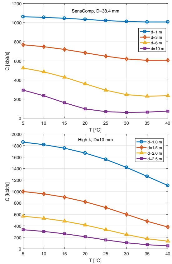
Fig. 5. Theoretical channel capacity as a function of temperature ( h_r = 50\% , p_s = 1 atm)
