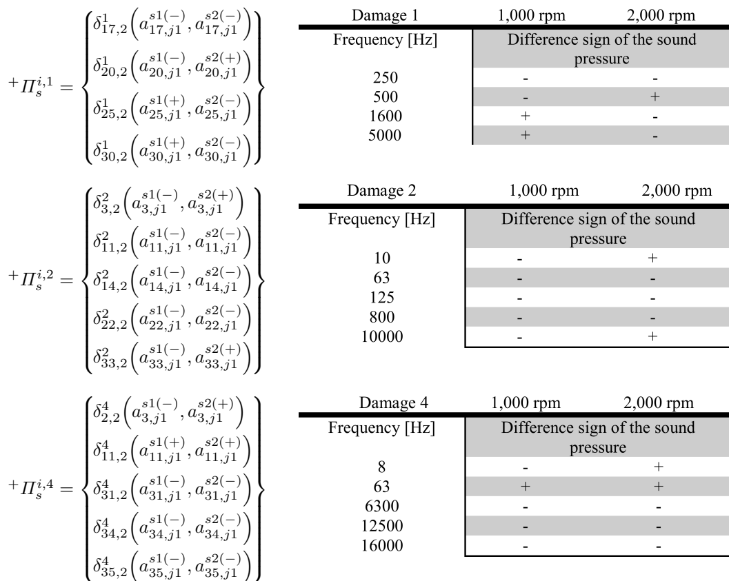
Fig. 12. Detection of engine damage based on sign comparison.
